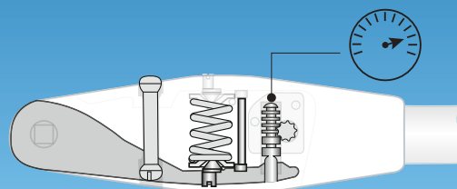
The working principle of the torque wrench with slave pointer type ADS-EDS
